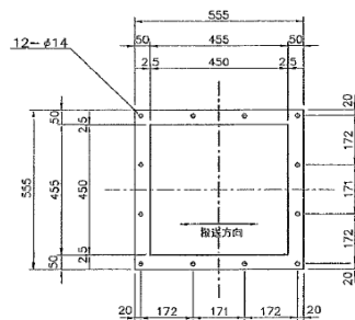
outlet flange (S=1/10) 10
