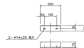
roller shaft (S=1/10) 11
