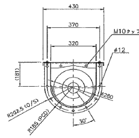
U-320 flange (S=1/10) 8
